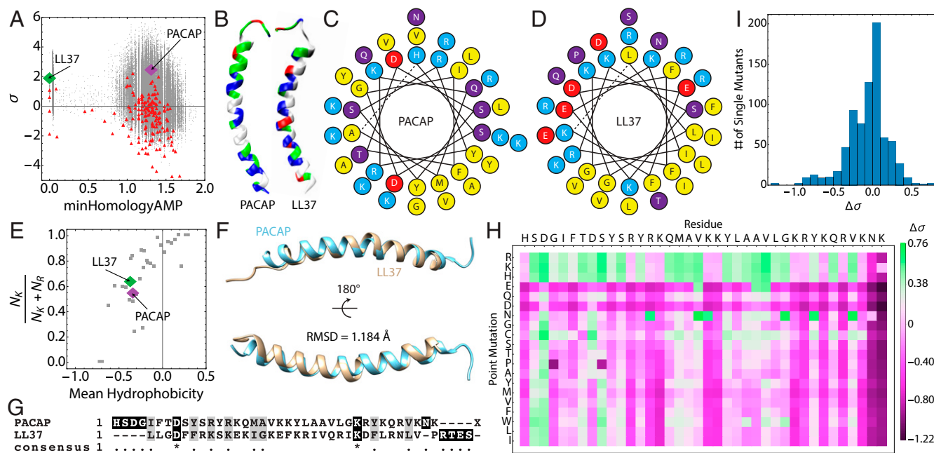
Fig. 1. PACAP is a GPCR-binding neuropeptide with strong physicochemical homology to human cathelicidin from innate immunity. (A) Screening a neuropeptide database (red) using the support vector machine-based MAPT for sequences with hidden membrane-restructuring activity revealed PACAP (purple) to be a hypothesized endogenous HDP. LL37 (green) is shown for comparison alongside sequences generated by a Monte Carlo-based directed search of sequence space (gray). (B) Comparison of the distribution of residue character along the lengths of PACAP and LL37 (blue = cationic, green = hydrophilic, white = hydrophobic, red = anionic). Helical wheel diagrams of (C) PACAP and (D) LL37 show similar distributions of hydrophobic (yellow) and cationic residues (teal). Anionic amino acids (red) and polar amino acids (purple) are also shown. (E) PACAP and LL37 exhibit similar lysine-to-arginine ratios and mean hydrophobicities, which suggests that PACAP (purple) can generate negative Gaussian membrane curvature similar to LL37 (green) and other \alpha -helical AMPs (gray). (F) Structural alignment of PACAP and LL37 yields an rmsd of 1.184 Å, demonstrating close structural similarity, despite (G) very low sequence homology. (H and I) An in silico mutational analysis of the entire PACAP sequence demonstrates that PACAP is locally optimized for membrane-remodeling activity, and that the majority of mutations reduce the microbicidal potential of the peptide.
